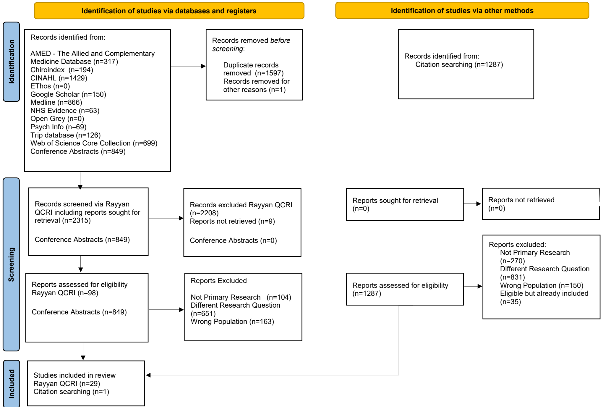
Figure 1: PRISMA 2020 flow diagram
